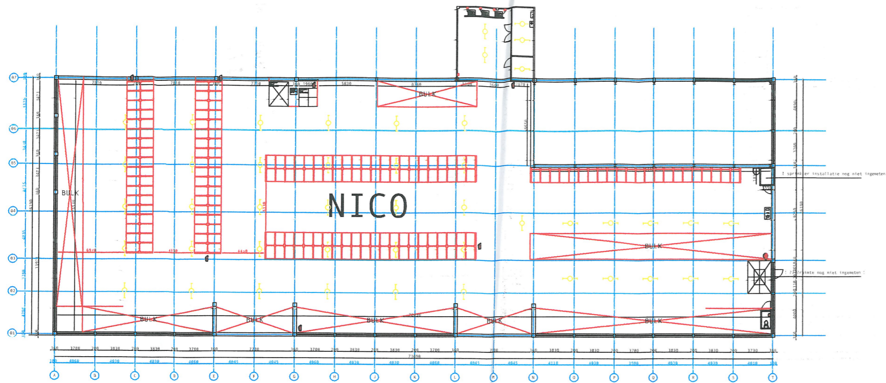
Plattegrond "NICO" Begane grond
